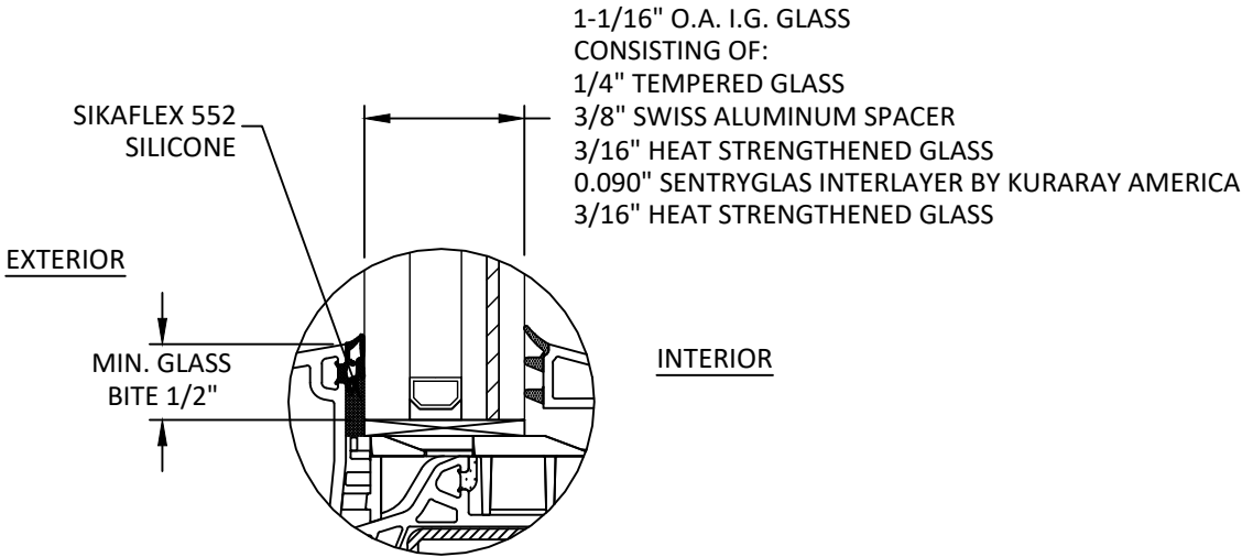
GLAZING DETAIL
